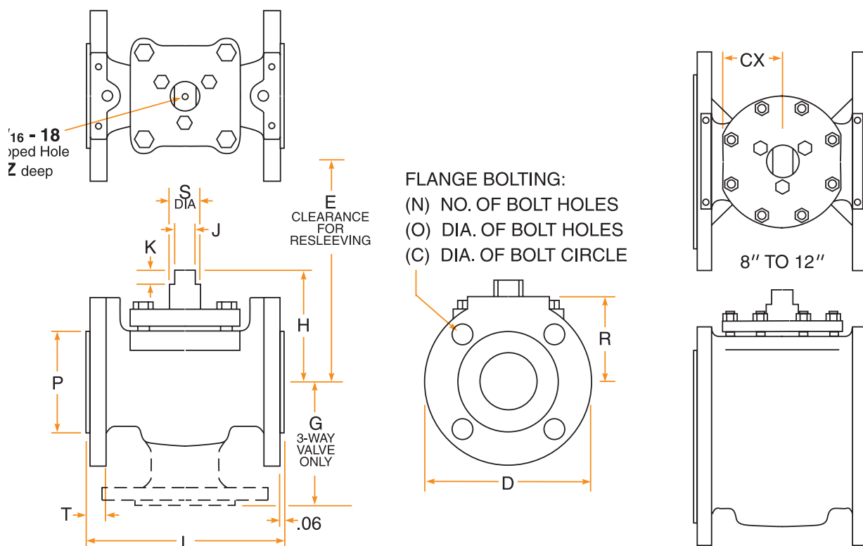
Flanged End / Class 150 / 2-Way - Figure No. 067 & 3-Way Figure No. 037
