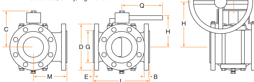
Class 150, 3-way, Fig. No. 031
