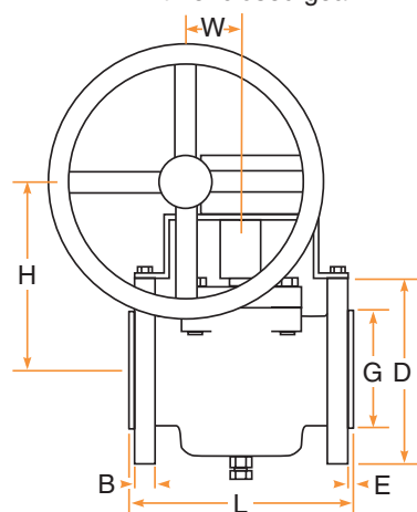
Class 150, 2-way, Fig. No. 061 with enclosed gear
