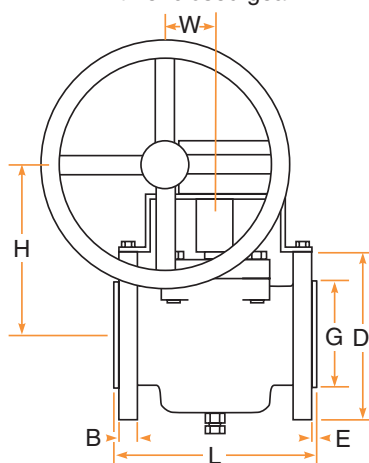
Class 300, 2-way, Fig. No. 0361 with enclosed gear
