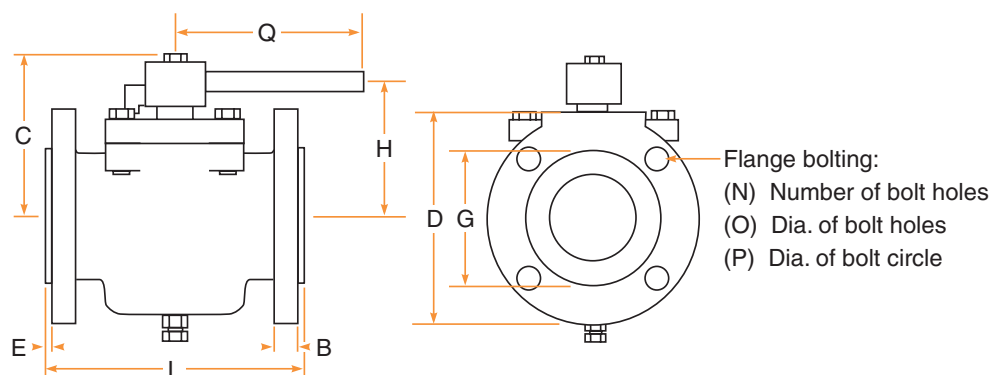
Class 300, 2-way, Fig. No. 0361
