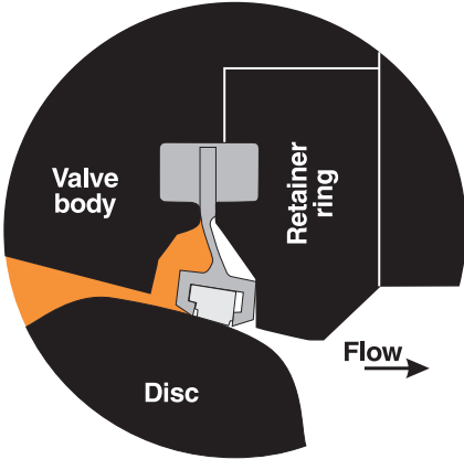
Normal operation - left to right flow.
