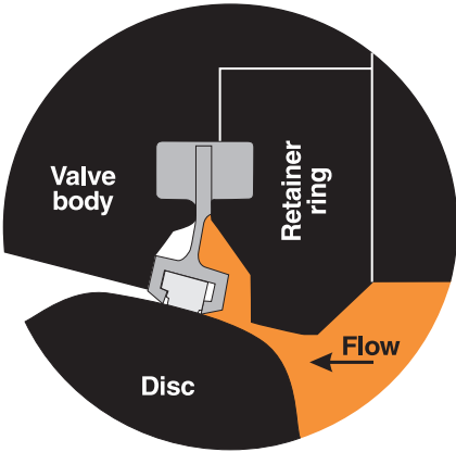
Normal operation - right to left flow.
