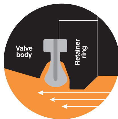
Figure 3. Valve open, with media flowing.
