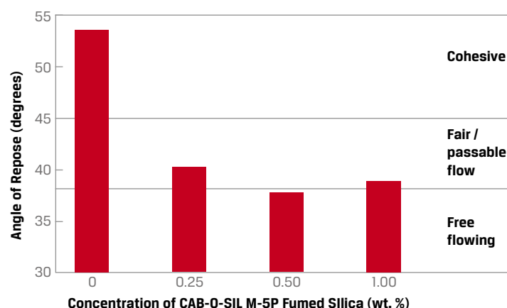
FIGURE 2: Effect of CAB-O-SIL M-5P fumed silica on APAP mixture flowability
