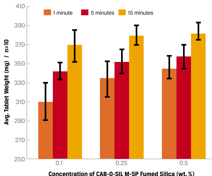
FIGURE 4: Effect of CAB-O-SIL M-5P fumed silica on tablet weight at various concentrations & mixing times
