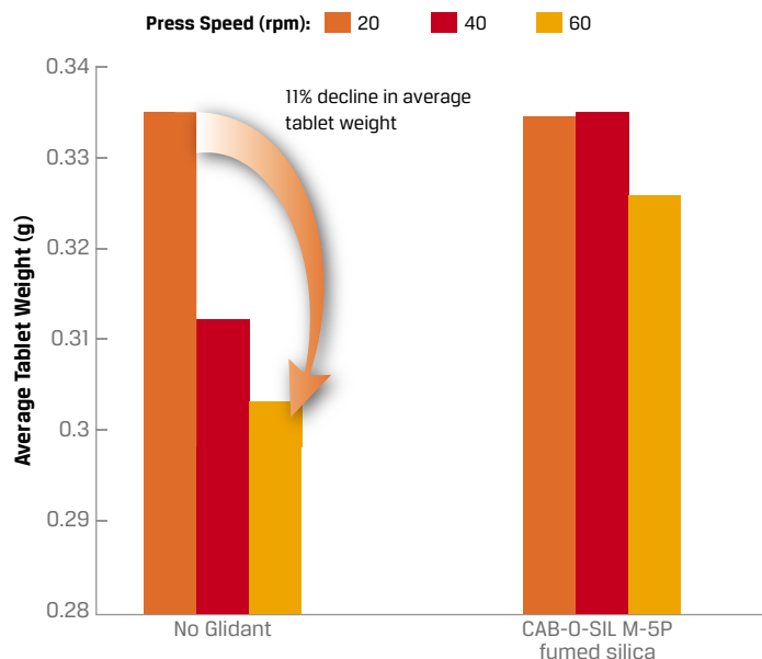
FIGURE 5: Effect of CAB-O-SIL M-5P fumed silica & press speed on tablet weight
