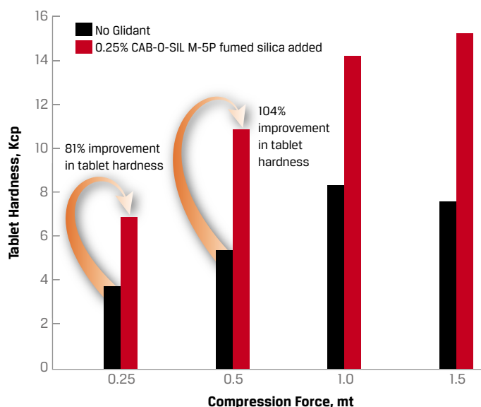
FIGURE 8: Effect of CAB-O-SIL fumed silica on tablet hardness at various compression force levels
