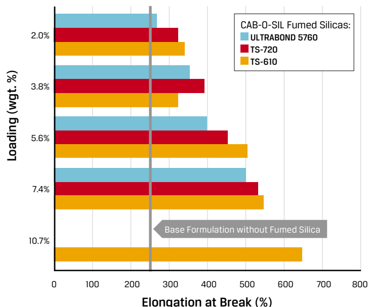
Effect of Fumed Silica on Elongation (in 1K PU Adhesive)
