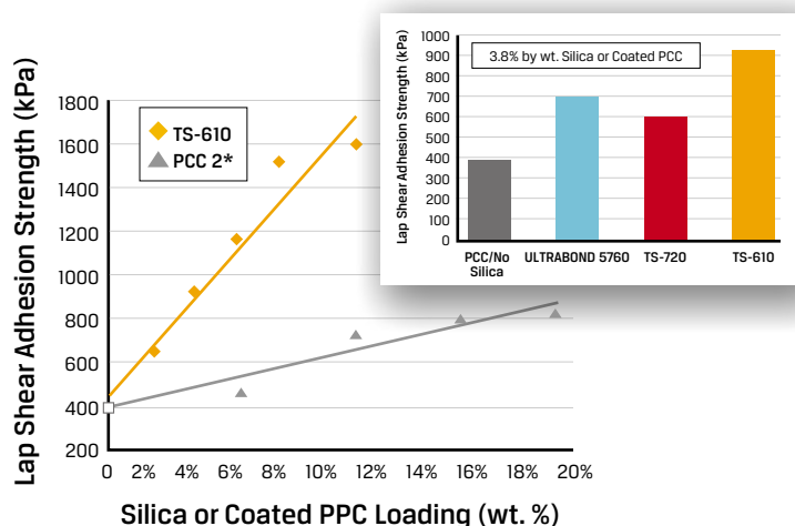
Effect of Fumed Silica and Coated Precipitated Calcium Carbonate (PCC) on Lap Shear Strength (in 1K PU Adhesive)
