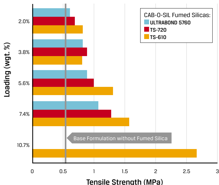
Effect of Fumed Silica on Tensile Strength (in 1K PU Adhesive)
