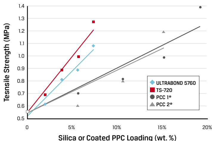
Performance Comparison of Coated Precipitated Calcium Carbonate (PCC) with PDMS-treated Silicas (in 1K PU Adhesive)
